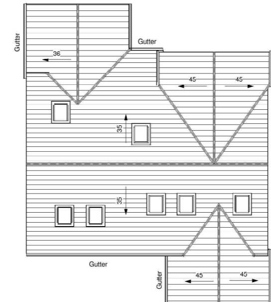
Proposed Roof Plan 1 : 100
